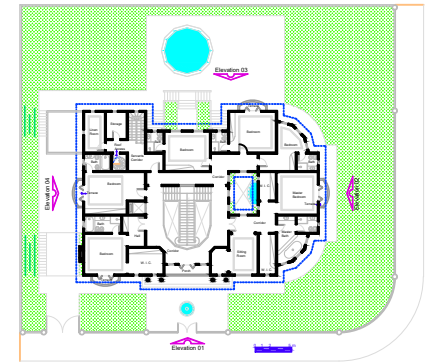
Second Floor Plan A = 367,89 m 2
