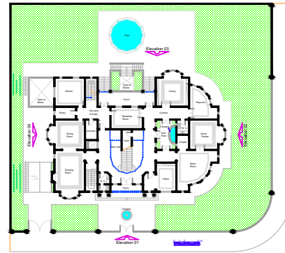
First Floor Plan A = 398,19 m 2
