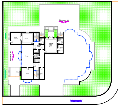
Lower Floor Plan A = 190,76 m 2
